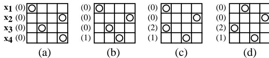
Figure 7. Example of an Algorithm Execution (Asynchronous Weak-commitment Search)
